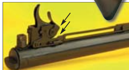
The trigger/safety unit and anti-beartrap link which ensures the gun can't inadvertently go off whilst loading. Top security from SMK!
